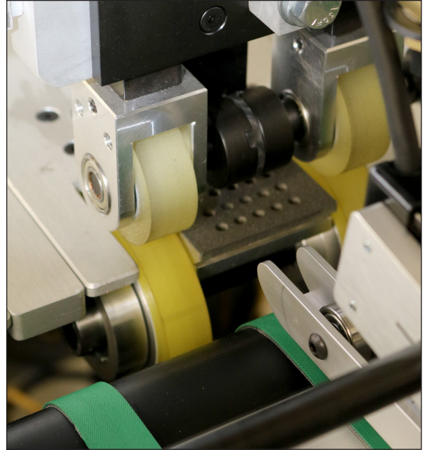
Adjustable feed rollers and vacuum plate.
